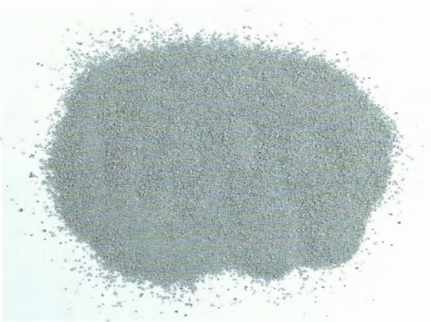
Figure 8.8 Dicalcium phosphate
